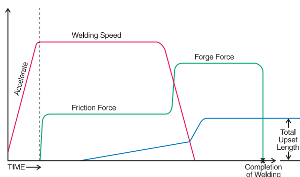
The relationship of direct-drive friction welding parameter characteristics.
