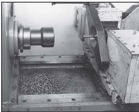
Above left: Model 120 Inertia Welder equipped with O.D. flash shearing.
