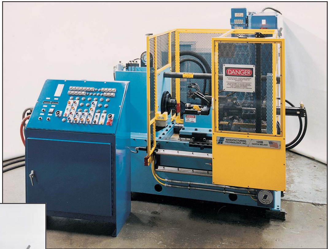
Model 120B Inertia Friction Welder Used to weld automotive air conditioning components.
